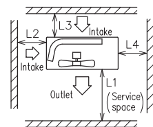
Minimum installation space
