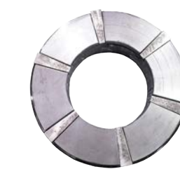
Thrust bearing - Direct lubrication type
