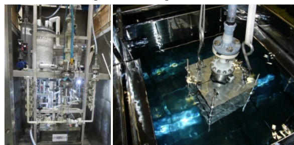
Figure 6: (left) BCP setup (right) Ultrasonic cleaning setup.
