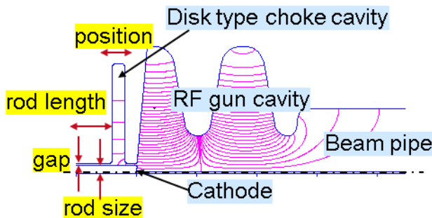
Figure 8: Cross section of RF gun cavity with choke cavity by SUPERFISH.
