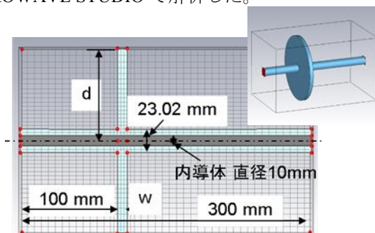
Figure 6: Cross section of disk type choke cavity and coaxial RF wave guide by MICROWAVE STUDIO.
