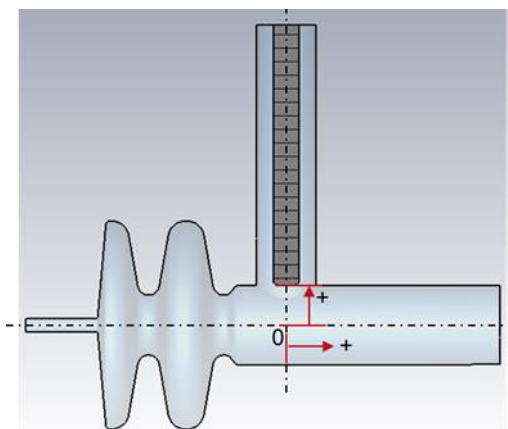
Figure 1: Cross section of initial gun cavity with RF coupler by MICROWAVE STUDIO.
